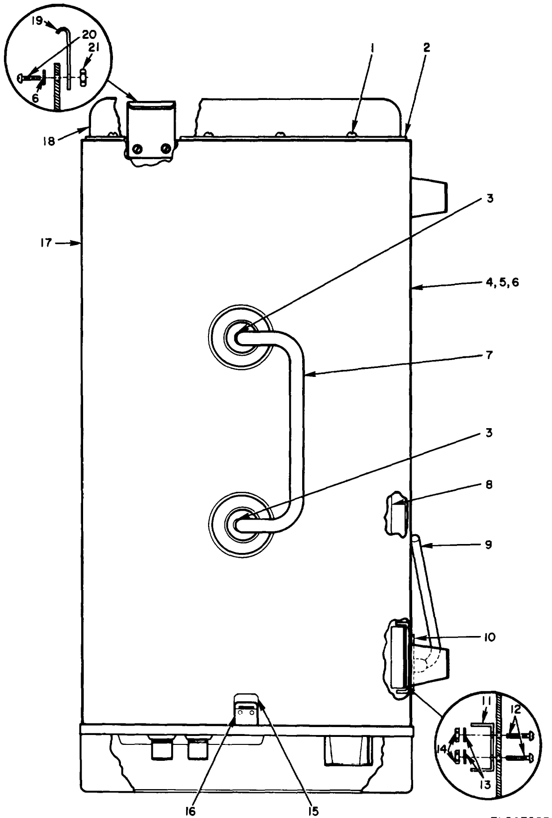
Figure 3. Meter, Modulation ME-505, Right View
