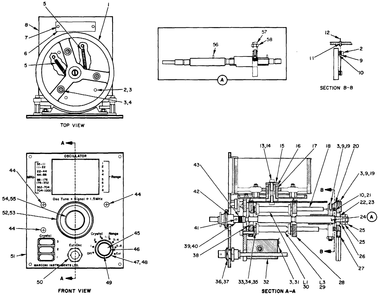
Figure 7. Oscillator, Front View
