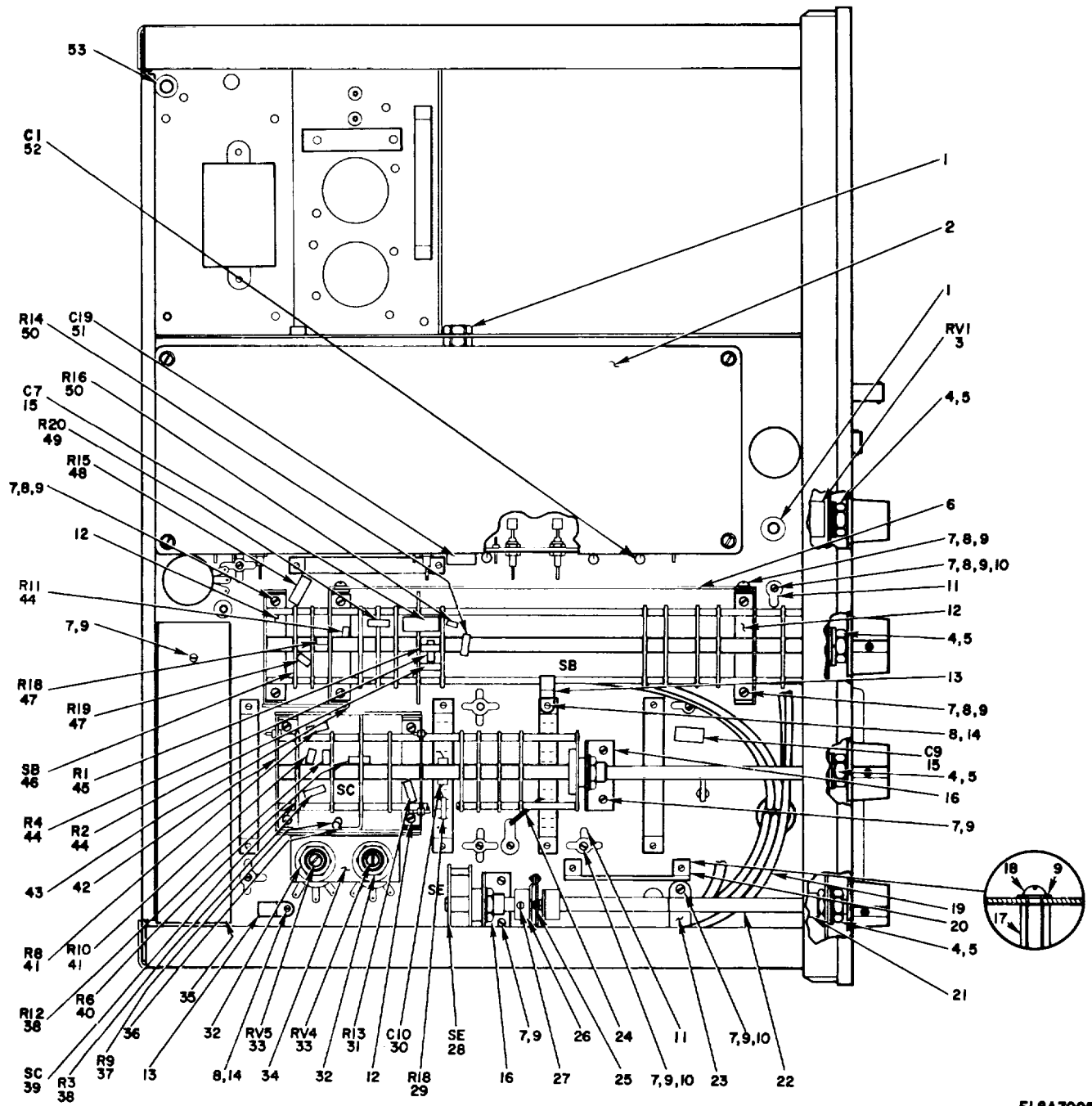
Figure 5. Meter, Modulation ME-505, Bottom View
