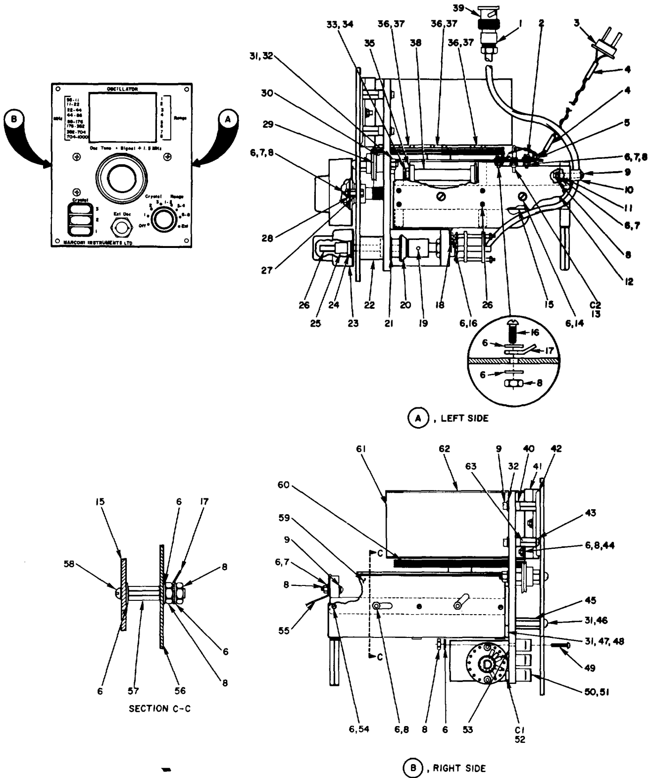
Figure 8. Oscillator, Left and Right View
