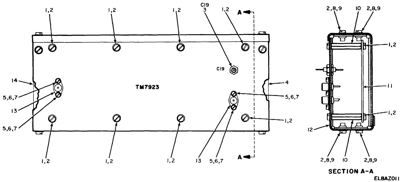
Figure 11. IF Amplifier
