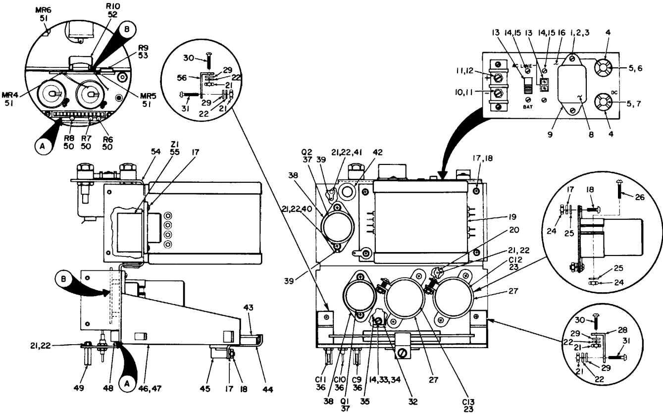
Figure 23. Power Supply Board, A13
