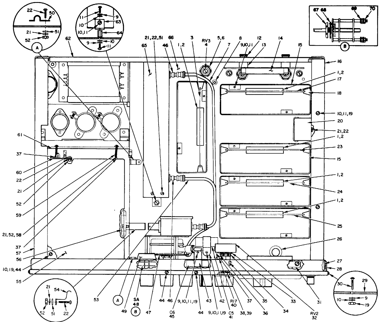
Figure 4. Meter, Modulation ME-505, Top View
