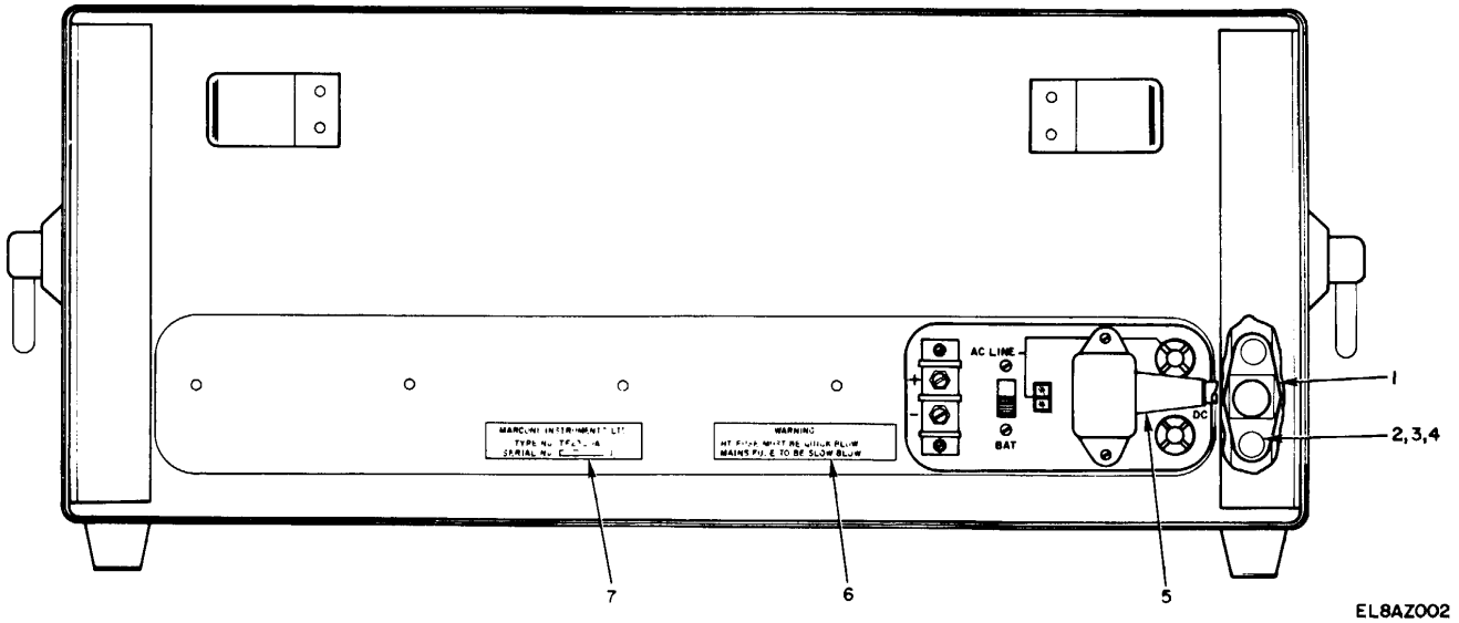
Figure 2. Meter, Modulation ME-505, Back View
