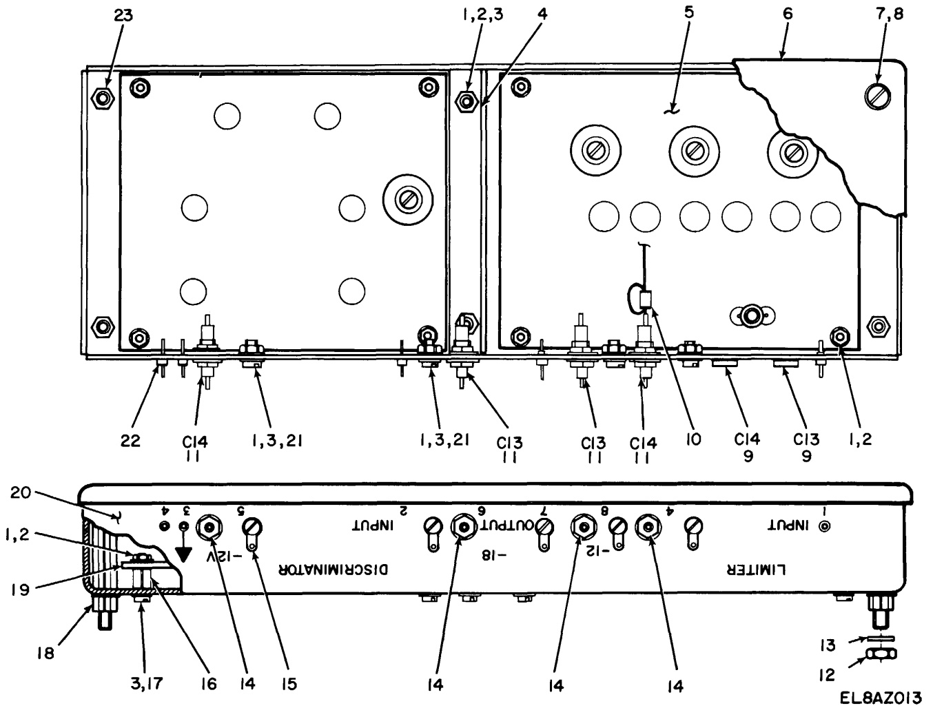
Figure 13. Limiter and Discriminator
