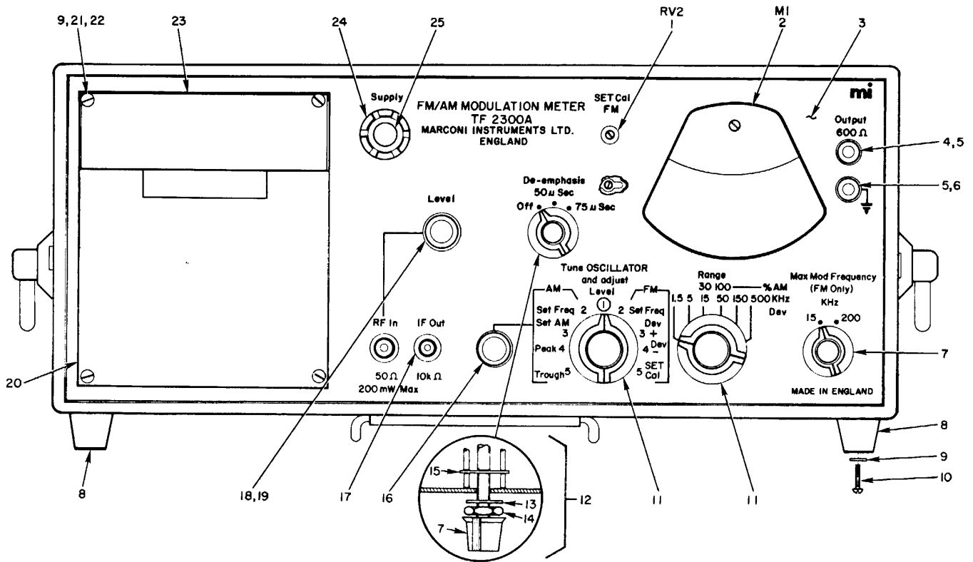
Figure 1. Meter, Modulation ME-505, Front View
